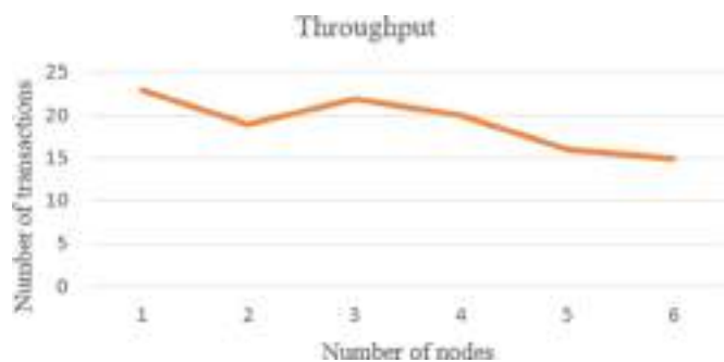
Fig. 7. Relationship between the number of nodes and throughput
