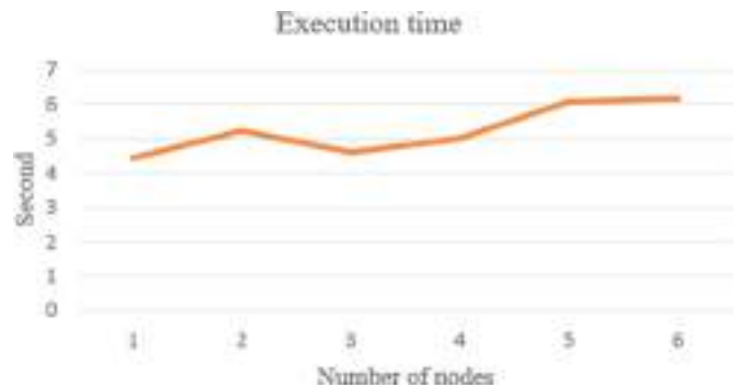
Fig. 6. Relationship between the number of nodes and execution time
