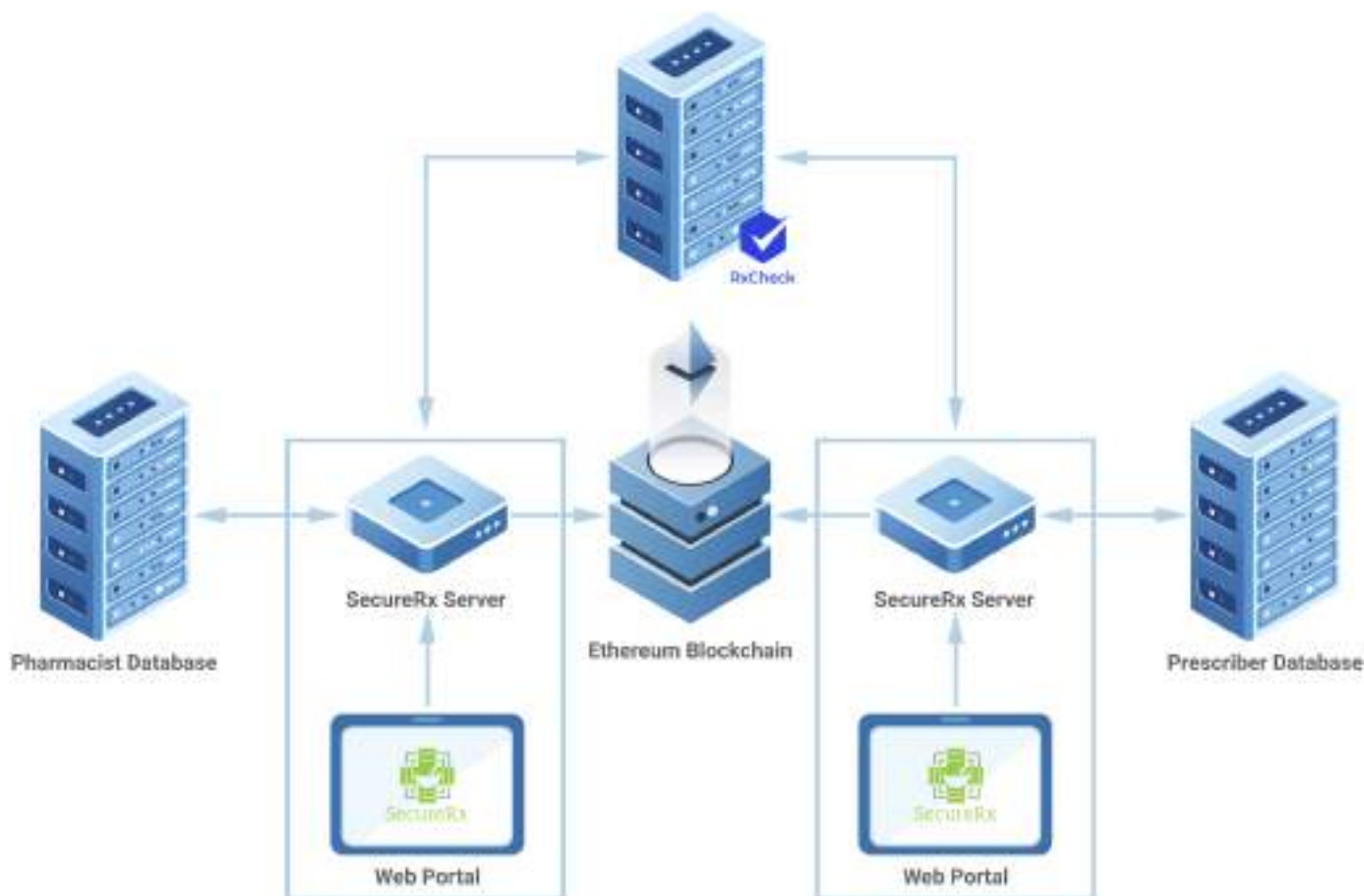
Fig. 1. SecureRx Architecture
